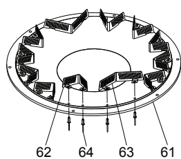
DISTRIBUTOR COVER 36/12 OUTPUTS
